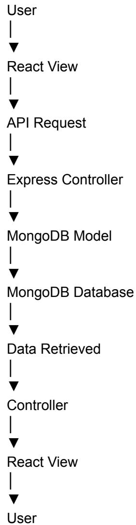
Figure 2: MVC Request Flow
